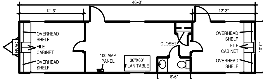
1050MORR 10' x 46' Box Size with 1/2 restroom
