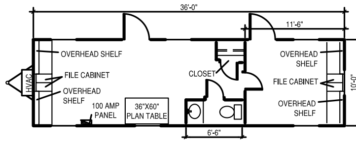
1040MORR 10' x 36' Box Size with 1/2 restroom
