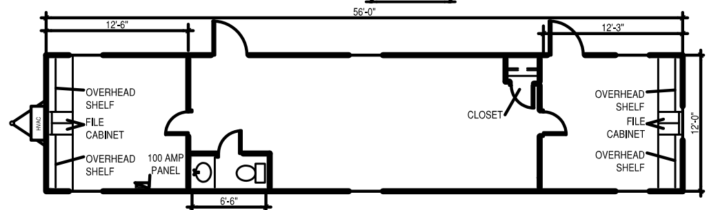
1260MORR 12' x 56' Box Size with 1/2 restroom
