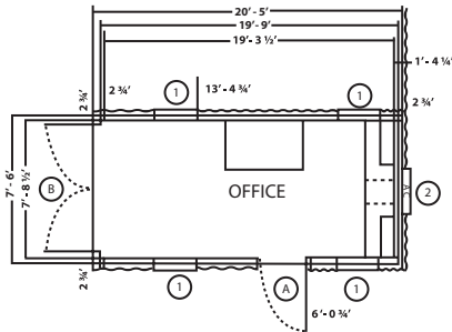
Example of available floor plan
