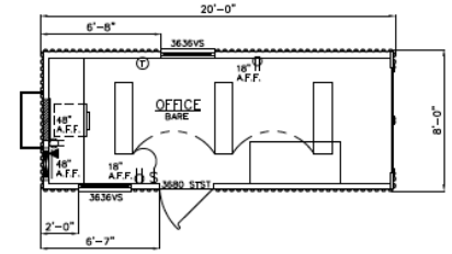
Example of available floor plan
