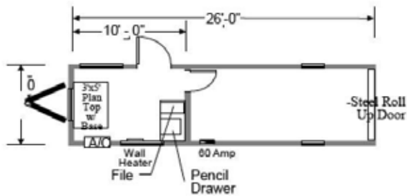
830MSO 8' x 26' Box Size Available with restrooms
